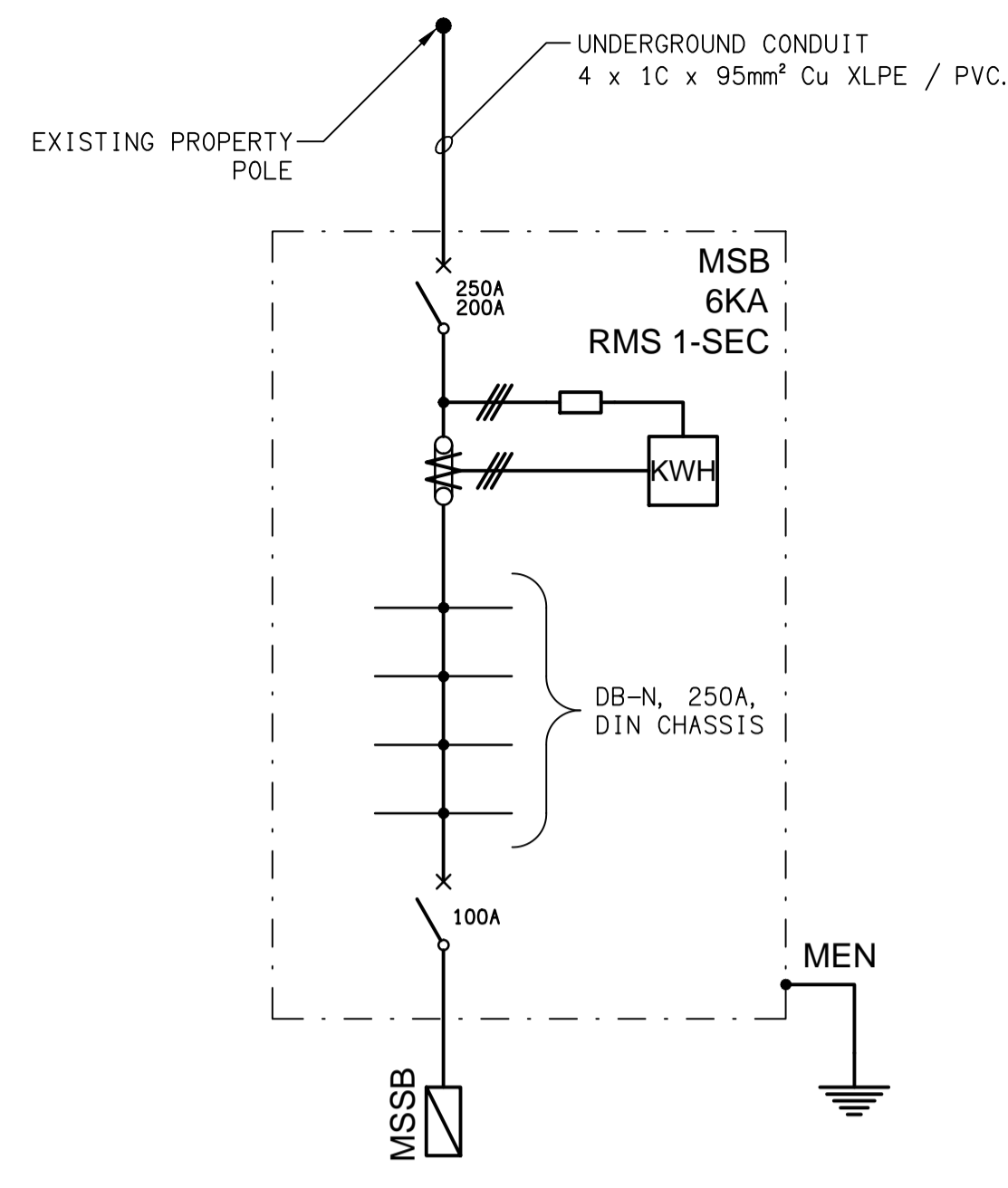
EXISTING SCHEMATIC POWER CONFIGURATION NOT TO SCALE
