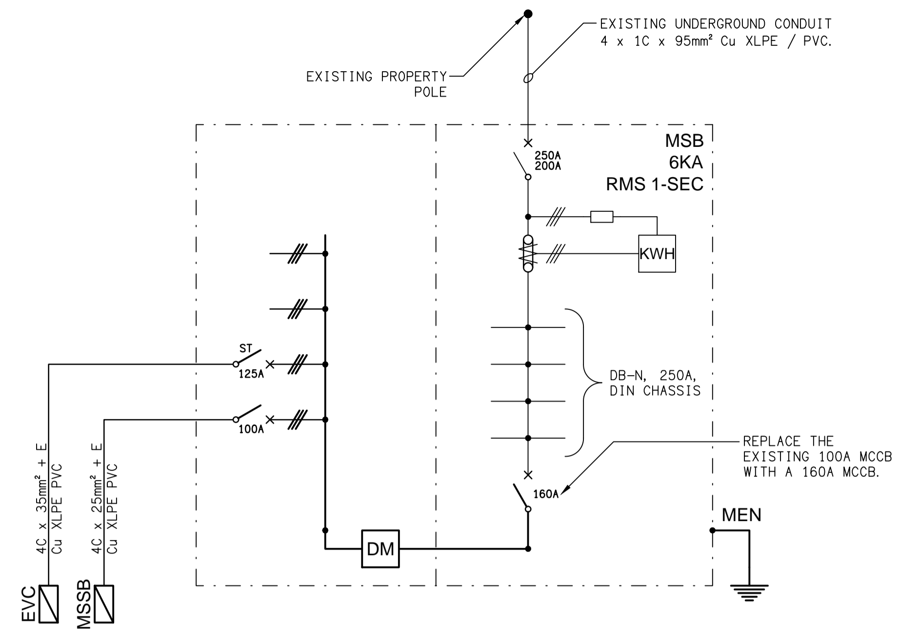
PROPOSED SCHEMATIC POWER CONFIGURATION NOT TO SCALE
