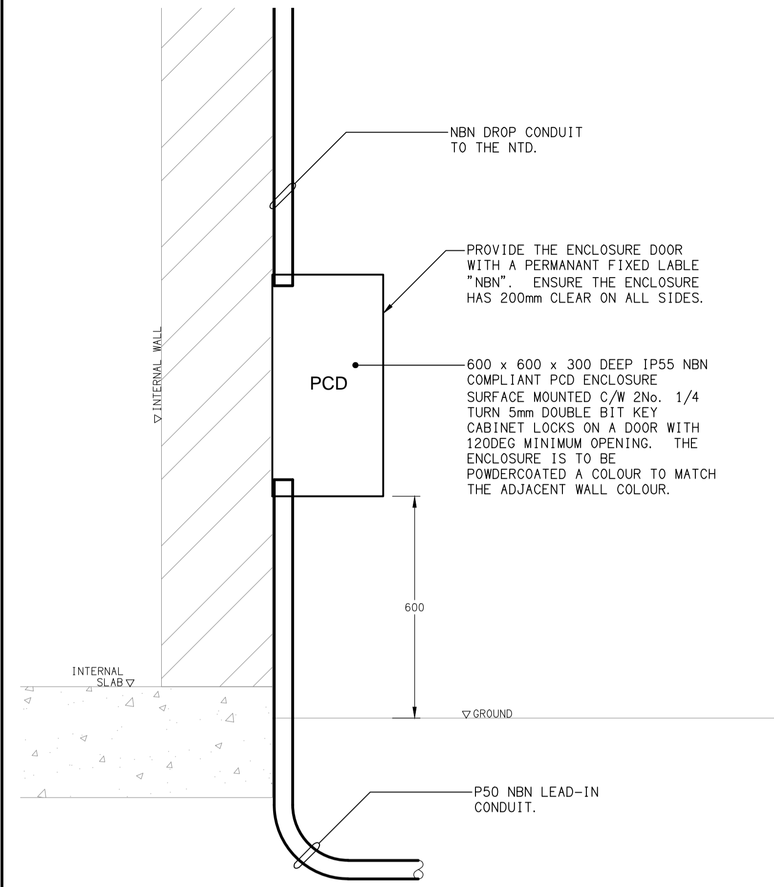
DETAIL PCD MOUNTING NOT TO SCALE
